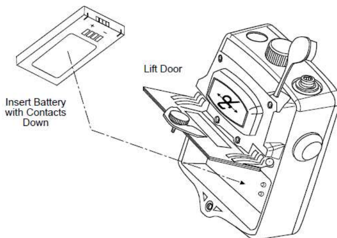
Figure 4: Battery Insertion/Removal
