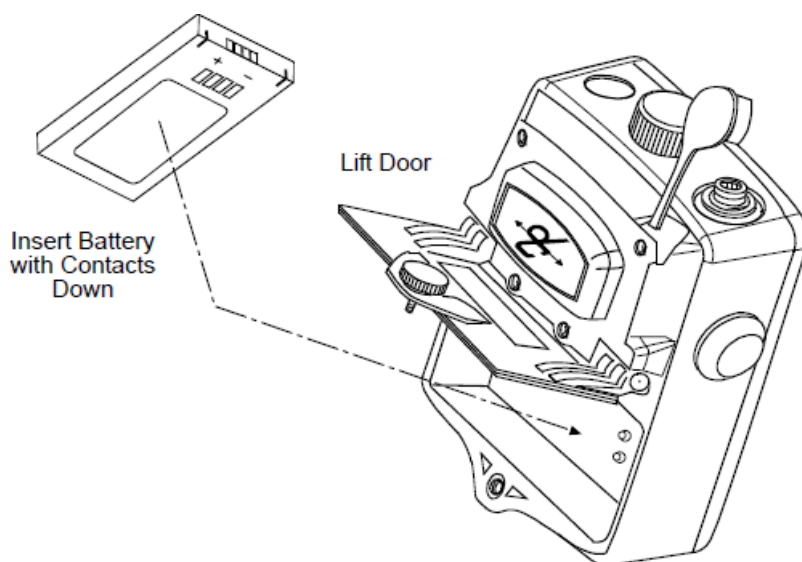
Figure 4: Battery Insertion/Removal
